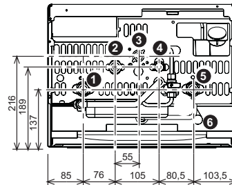
fig. 17 - Plumbing connections
