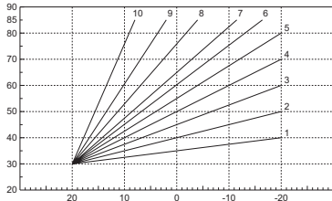
fig. 14 - Compensation curves
